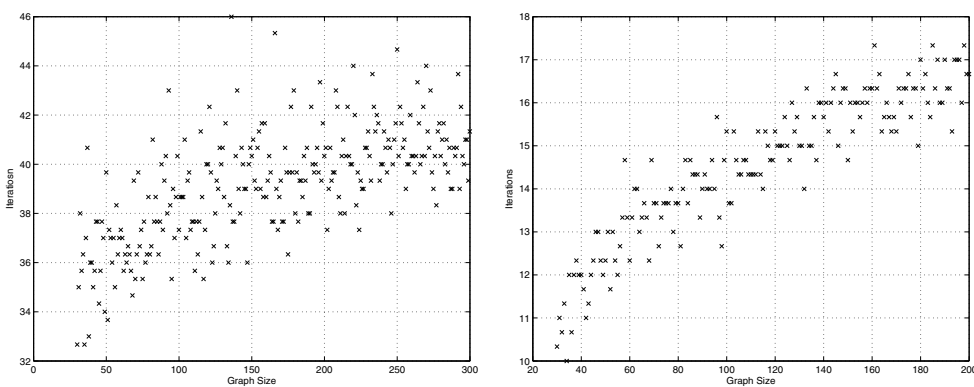
FIG. 9.2. On the left: Averaging in time-varying Erdős–Rényi random graphs with the load balancing algorithm. Here c = 3/4 at each time t . On the right: Averaging in time-varying geometric random graphs with the load balancing algorithm. Here r = \sqrt{\log n/n} .
