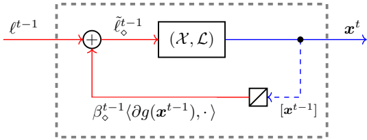
Figure 9. Regret circuit for the Lagrangian relaxation construction (Section 6.1) for the constrained set \mathcal{X} \cap \{\mathbf{x} : g(\mathbf{x}) \leq 0\} .
