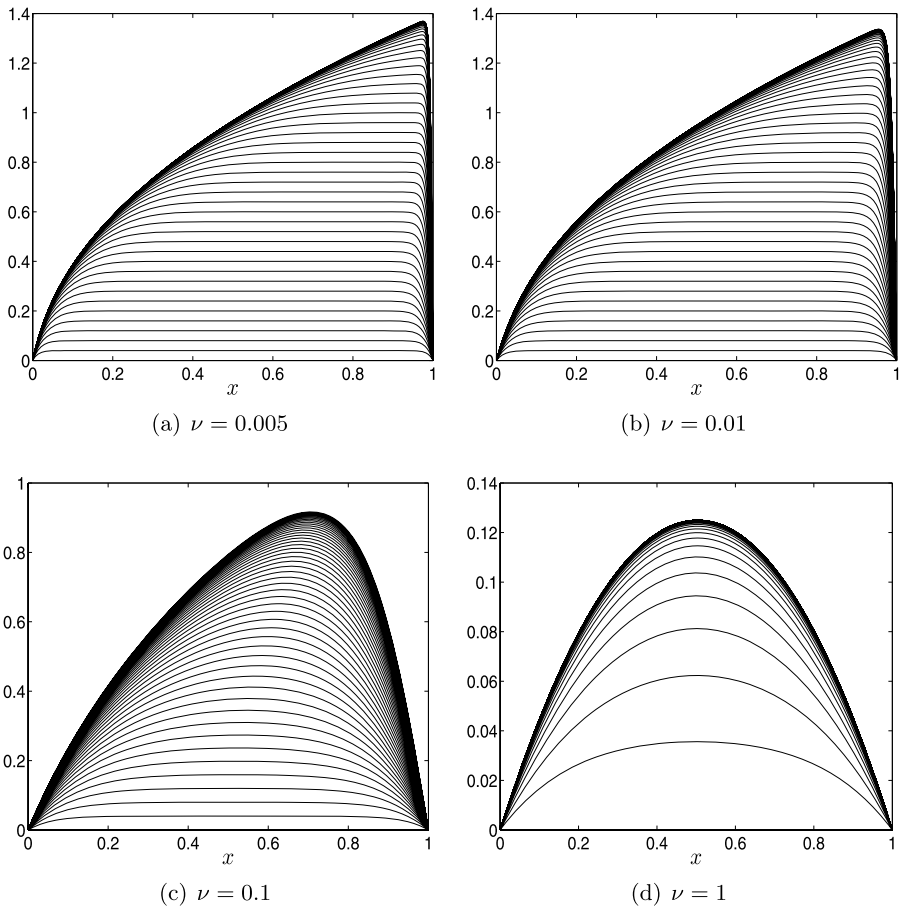
Fig. 1 Solution of the Burgers' equation u^{\mathcal{N}}(x, t^k; \nu) as a function of x and t^k : (a) \nu = 0.005 , (b) \nu = 0.01 , (c) \nu = 0.1 , and (d) \nu = 1
