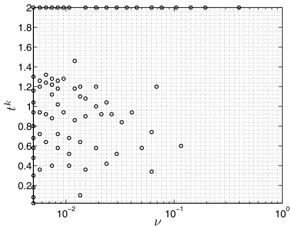
Fig. 3 Distribution of the SCM parameter sample \mathcal{C}_J in time (linear scale) and parameter (log scale). The grid represents \mathcal{E}_{\text{train,SCM}} : each horizontal gray line corresponds to a t^k, k = 2, 4, \dots, K ; each vertical gray line corresponds to a point in \mathcal{E}_{\text{train,RB}}
