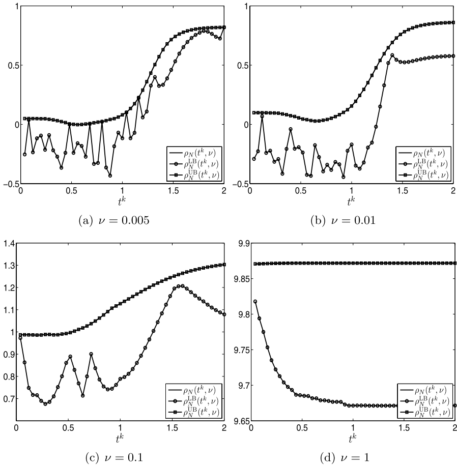
Fig. 4 Stability factors \rho_N(t^k; \nu) , \rho_N^{LB}(t^k; \nu) , and \rho_N^{UB}(t^k; \nu) as a function of t^k for N = 17 : (a) \nu = 0.005 , (b) \nu = 0.01 , (c) \nu = 0.1 , and (d) \nu = 1
