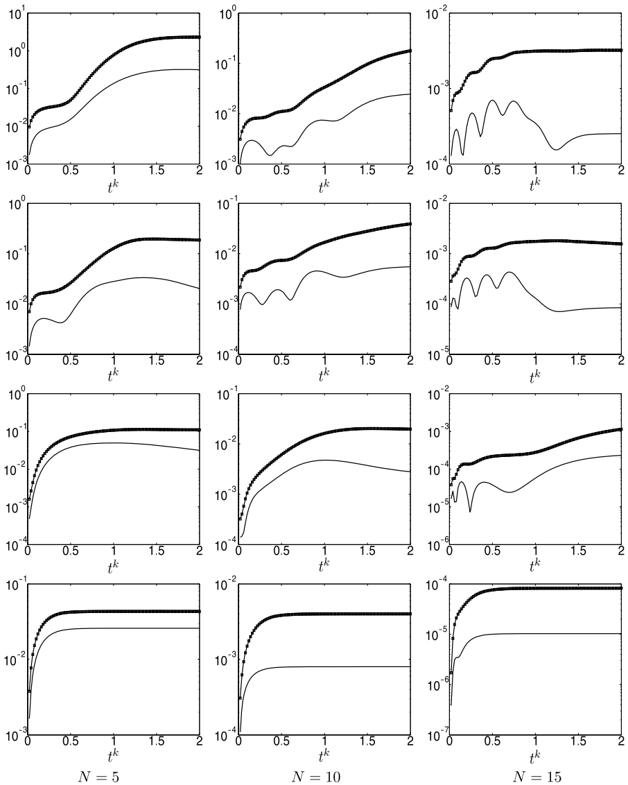
Fig. 5 The actual L^2(\Omega) error, \|u^{N^k}(\nu) - u_N^k(\nu)\| (solid line), and the L^2 error bound, \Delta_N^k(\nu) (square symbol), as a function of discrete time t^k for N = 5 (first column), 10 (second column), and 15 (third column) and for \nu = 0.005 (top row), \nu = 0.01 (second row), \nu = 0.1 (third row), and \nu = 1 (bottom row)
