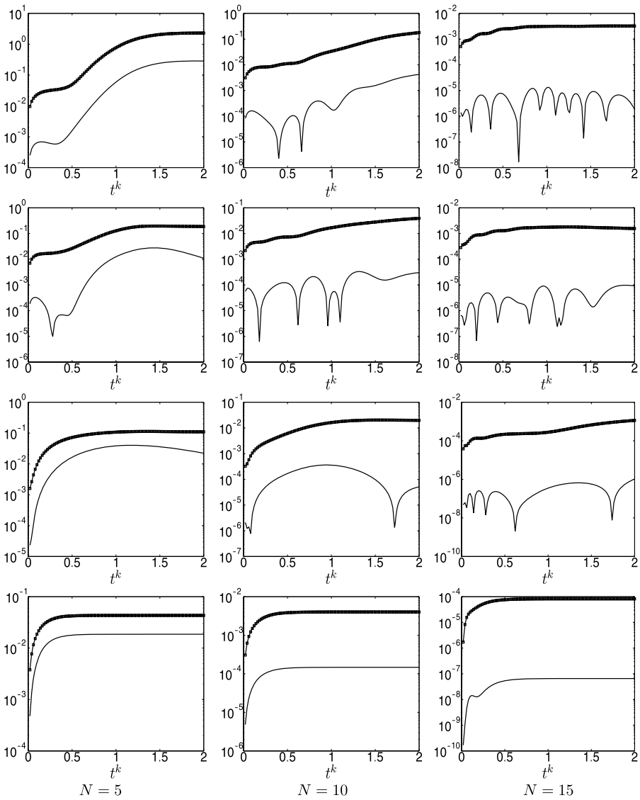
Fig. 6 The output error, |s^{\mathcal{N}^k}(\nu) - s_N^k(\nu)| (solid line), and the output error bound, \Delta_N^{s,k}(\nu) (square symbol), as a function of discrete time t^k for N = 5 (first column), 10 (second column), and 15 (third column) and for \nu = 0.005 (top row), \nu = 0.01 (second row), \nu = 0.1 (third row), and \nu = 1 (bottom row)
